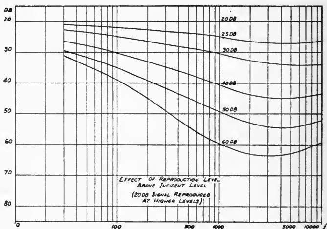
FIG. 2. Effect of reproduction level above incident level.
